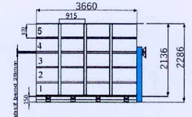
SYSTEM B 4 BAYS MOBILE COMPACTOR
