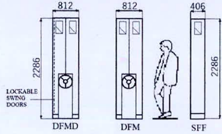
SYSTEM A & SYSTEM B FRONT ELEVATION
